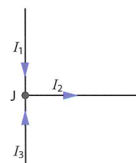
Figure 5.34 Currents at junction J.
