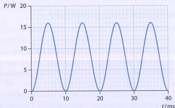
Figure 11.21 The variation with time of the power delivered by an ac generator.
