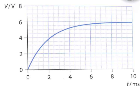
Figure 11.39 The variation of potential difference with time for a charging capacitor.
