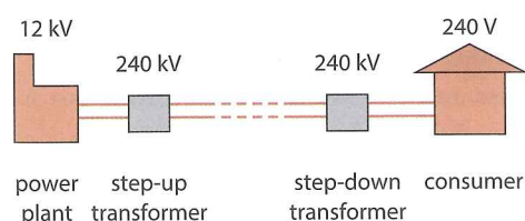
Figure 11.26 A schematic version of Figure 11.25.
