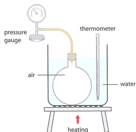
Figure 3.19 Investigating the pressure–temperature law.
