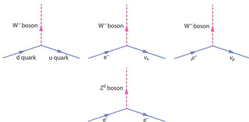
Figure 7.28 Weak interaction vertices.
