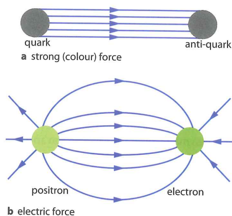
Figure 7.31 The lines of force between a quark and an anti-quark are very different from those between a positive and a negative electric charge, leading to quark confinement.
