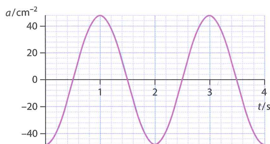
Figure 4.6 The variation of acceleration a with time t in SHM.
