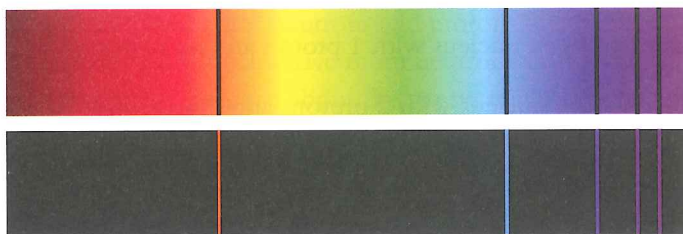
Figure 7.5 The absorption spectrum of hydrogen (top) and the emission spectrum (bottom). The emission lines and the absorption lines are at the same wavelength.
