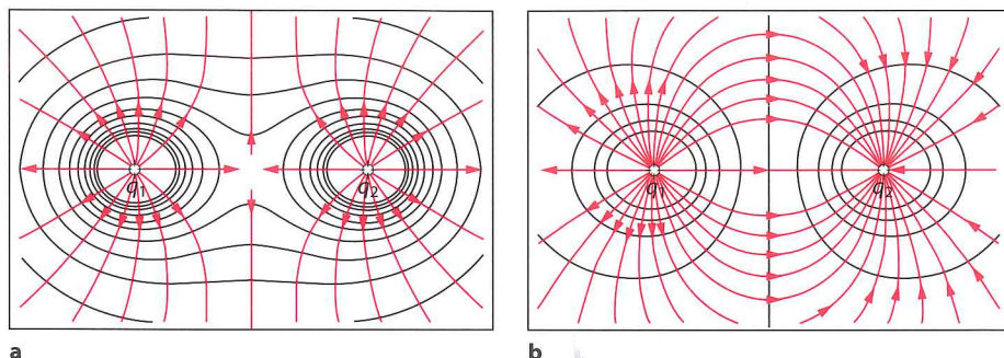
Figure 10.22 Field lines and equipotential surfaces for a two equal charges of the same sign and b two equal and opposite charges.
