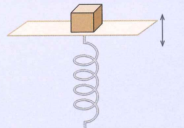
Figure 9.5 A particle on a horizontal plate executing SHM.
