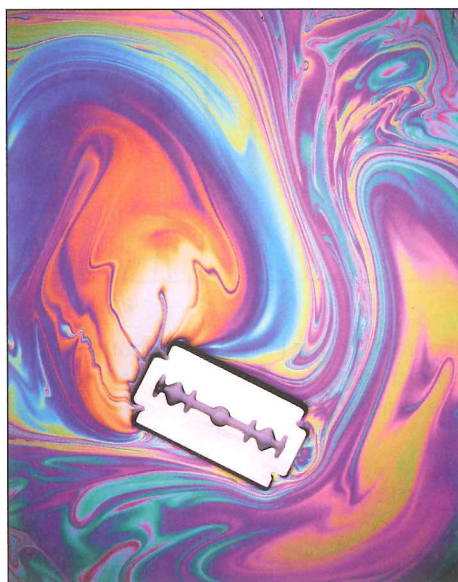
Figure 9.27 Interference pattern in a thin film of oil floating on water.
