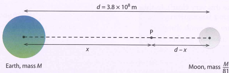
Figure 10.7 The Earth-Moon system.
