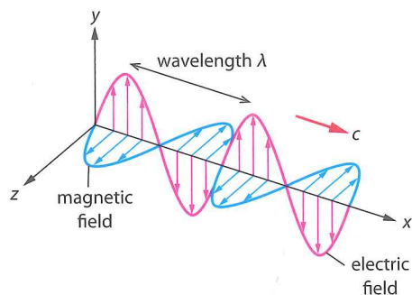
Figure 4.25 An EM wave propagating along the direction of the x -axis. The electric and magnetic fields are in phase, i.e. they have matching crests, troughs and zeroes. The two fields are at right angles to each other at all times.
