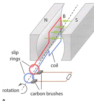
Figure 11.15 a A coil that is forced to turn in a region of magnetic field will produce an emf. b Generators at the Hoover hydroelectric power plant in the USA.
