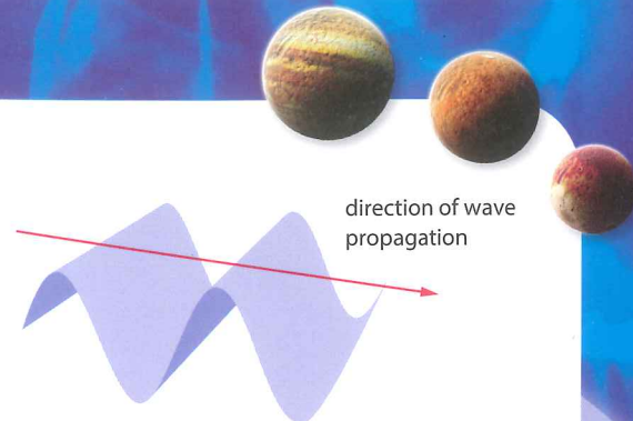
Figure 4.27 A two-dimensional wave.
