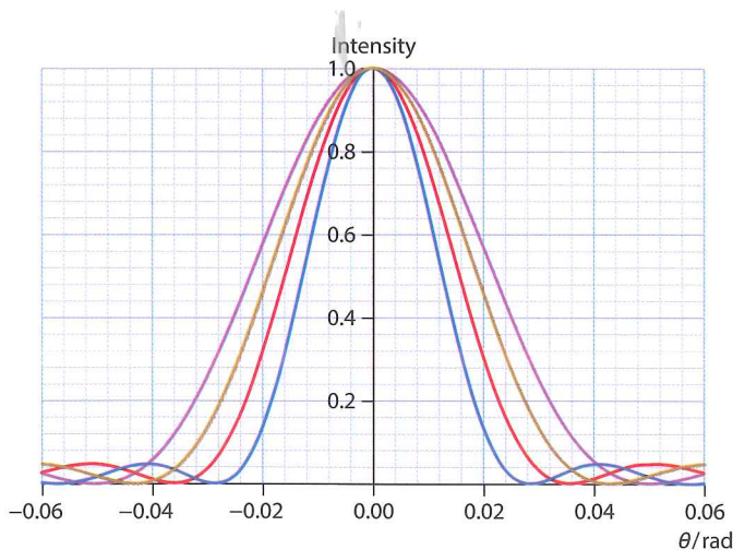
Figure 9.15 The single-slit intensity pattern for white light. The central bright spot is white but the rest of the pattern is coloured.
