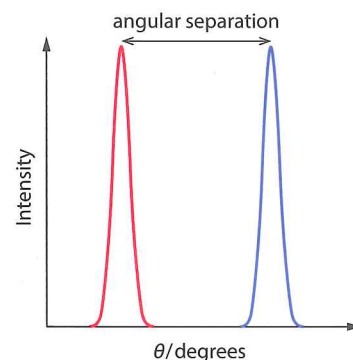
Figure 9.35 Two lines that are close to each other may not be resolvable.
