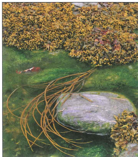
Figure 4.44 The reflected light from the water is reduced when observed through a vertical polariser. This allows detail inside the water (the vegetation and pebbles) to be seen more clearly.
