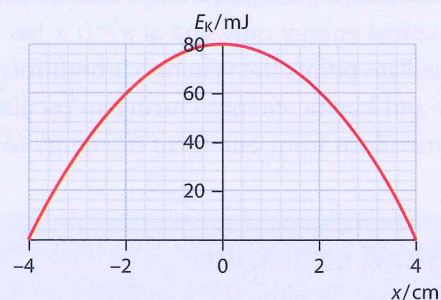
Figure 9.8 The variation with displacement of the kinetic energy of a particle.
