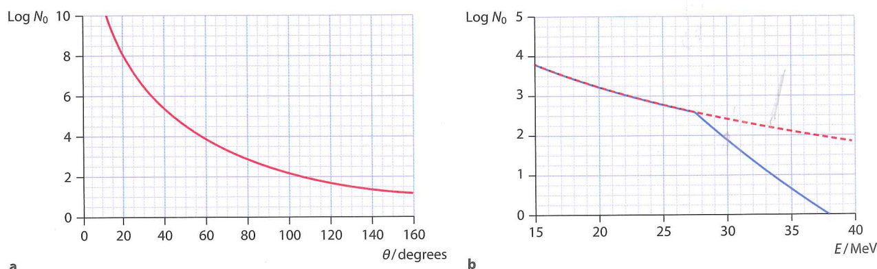
Figure 12.23 a The logarithm of the number of alpha particles scattered at some angle \theta as a function of \theta . b The logarithm of the number of alpha particles scattered at an angle of 60^\circ as a function of the alpha particle energy. The dotted curve is based on Rutherford scattering. The blue curve is the observed curve. We see deviations when the energy exceeds about 28 MeV. The energy at which deviations start may be used to estimate the nuclear radius.
