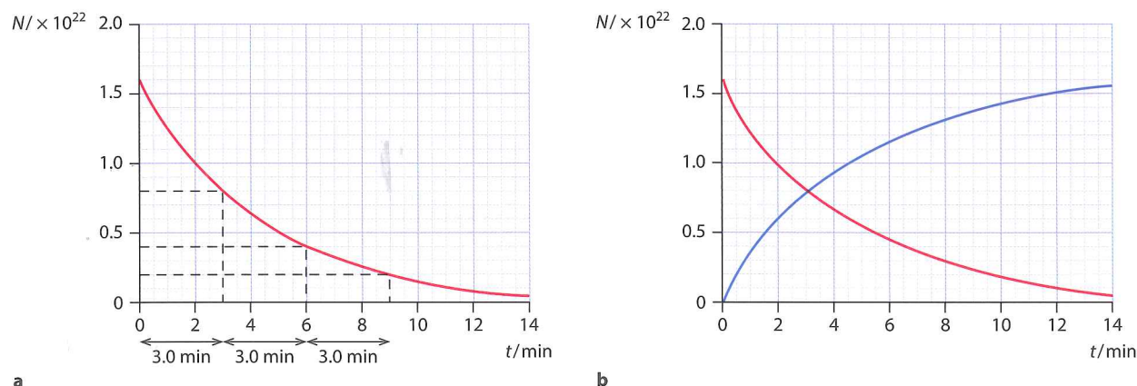
Figure 7.8 a The number of thallium nuclei decreases exponentially. b As thallium decays (red curve) lead is produced and so the number of lead nuclei increases (blue curve).
