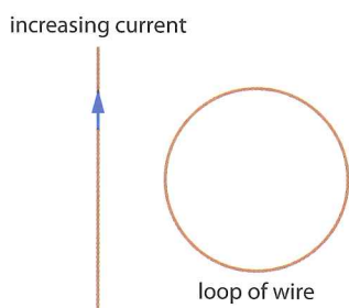
Figure 11.11 A loop of wire near a straight wire in which the current is increasing.
