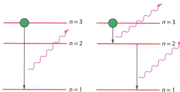
Figure 7.4 Transitions from n=3 in hydrogen.
