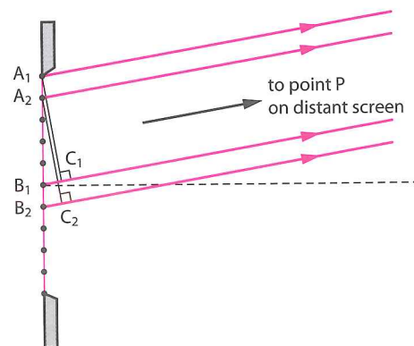
Figure 9.11 Triangles A_1B_1C_1 and A_2B_2C_2 are congruent.
