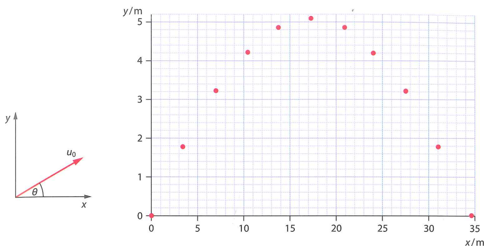
Figure 2.19 A launch at \theta = 30^\circ to the horizontal with initial speed 20 \text{ m s}^{-1} .
