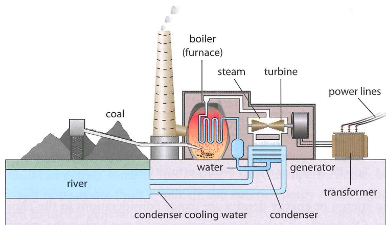
Figure 8.1 A coal-burning power plant.
