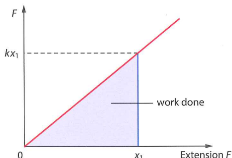
Figure 2.63 The force F stretches the spring. Notice that as the extension increases the force increases as well.
