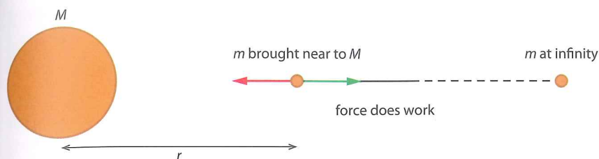
Figure 10.3 Work is done to bring the small mass from infinity to a given position away from the big mass. The red arrow is the force of attraction between the two masses. We are interested in the work done by the force represented by the green arrow, i.e. the work done by the external agent. This work is negative and is stored as potential energy. The work done is independent of the actual path followed.
